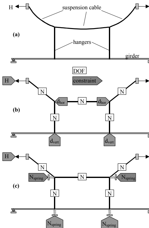
Figure 4: Optimisation for shape finding at suspension bridges
