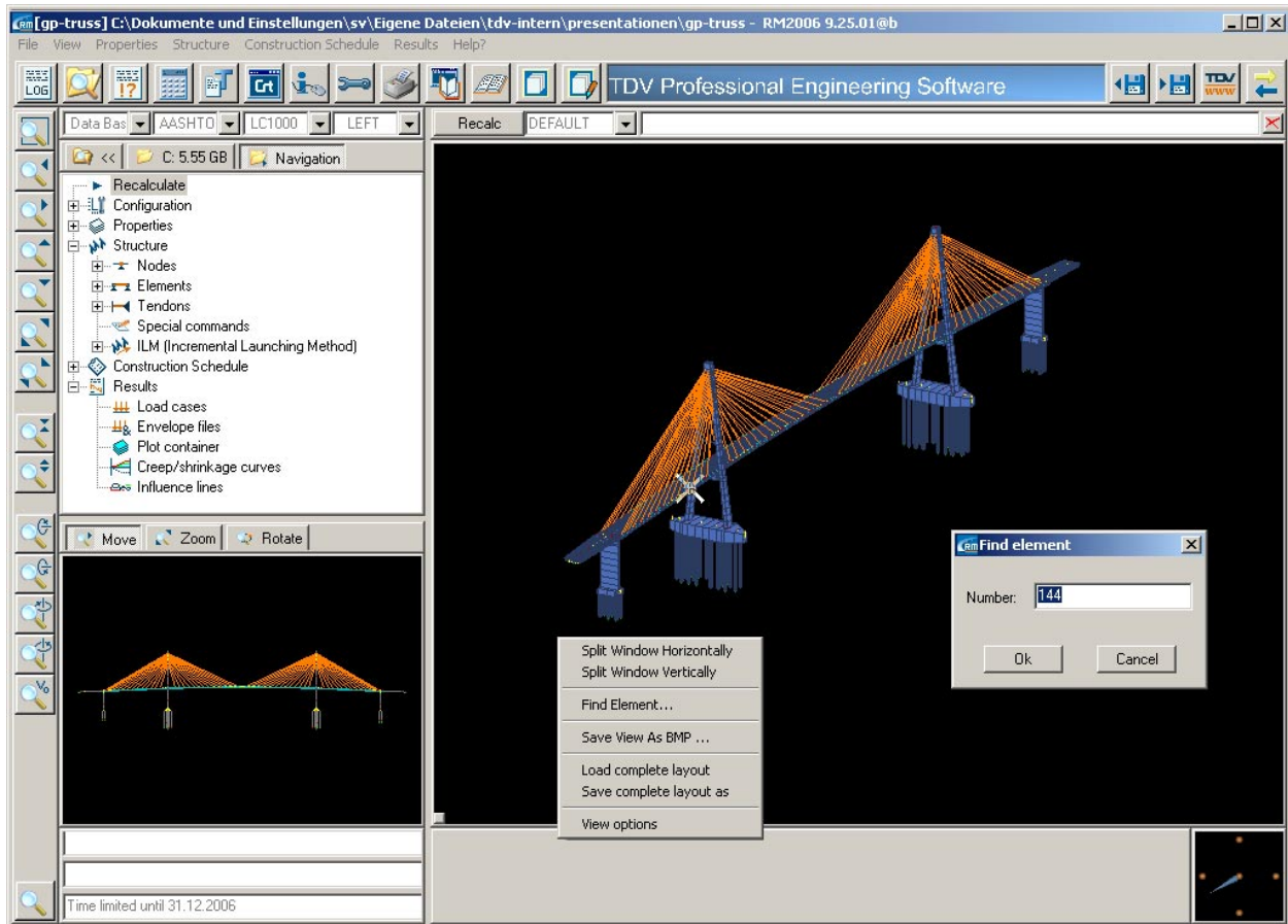
Figure 8: Improved GUI-handling
