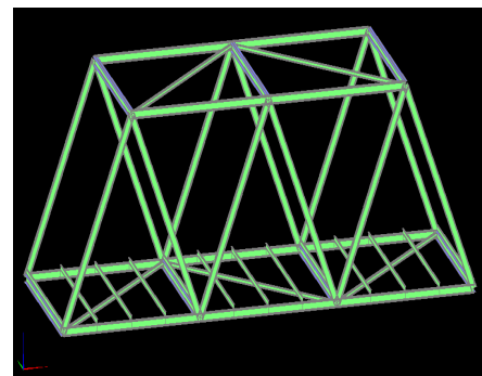
Figure 2: Truss modelling with link segments
