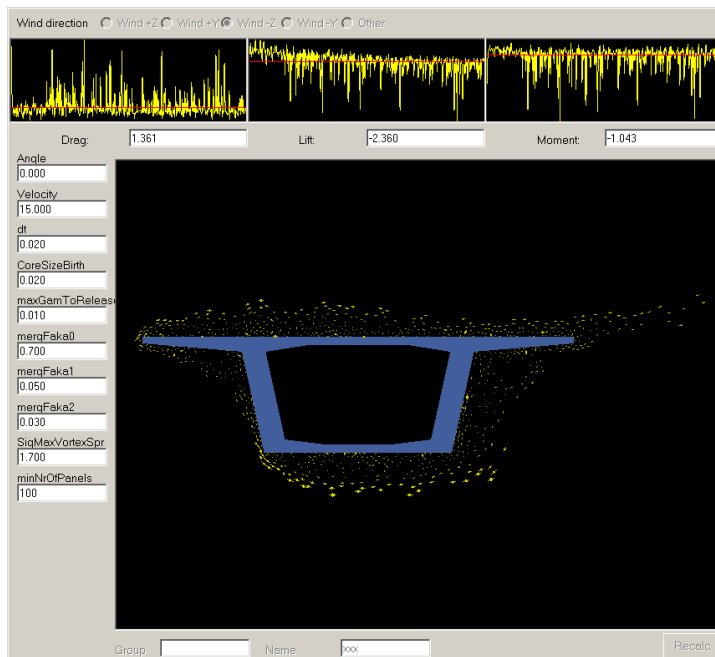
Figure 10: New RM2006 CFD module, based on the "Vortex particle" method
