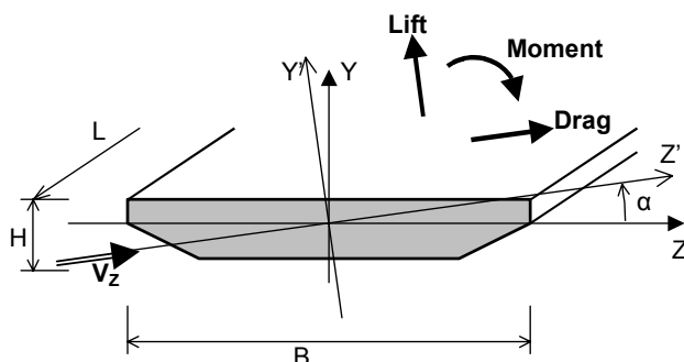
Figure 7: Wind forces action on the bridge section
