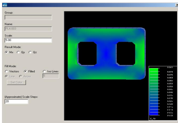
Figure 9: Local stress distribution
