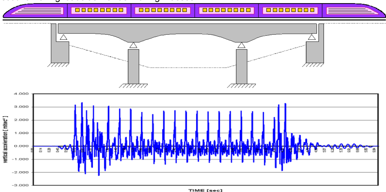
Figure 6: Structural accelerations due to passing of High Speed Train
